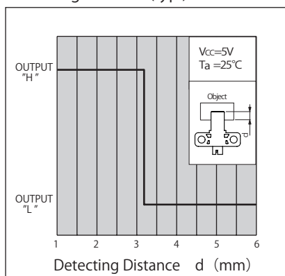
検出位置特性2 (代表例) KI5350 Detecting Distance (typ.)
