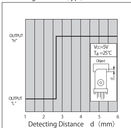
検出位置特性2(代表例) KI3991 Detecting Distance (typ.)
