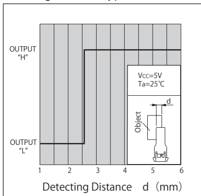
検出位置特性1 (代表例) KI5771 Detecting Distance (typ.)
