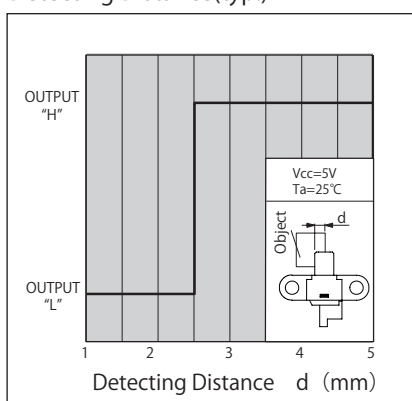
検出位置特性1 (代表例) KI5231 Detecting Distance (typ.)
