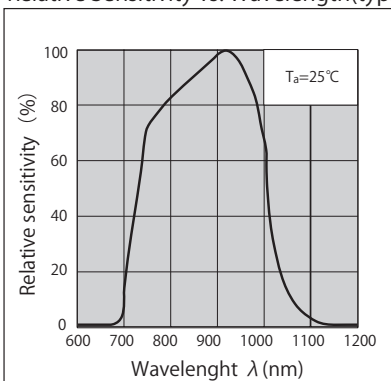
分光感度特性 (受光側) (代表例) Relative Sensitivity vs. Wavelength (typ.)
