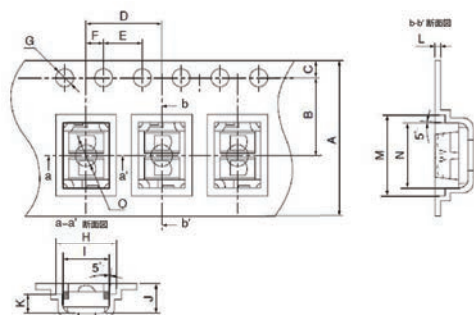
寸法表／Dimensions List
