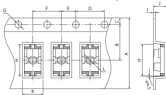
寸法表／Dimensions List
