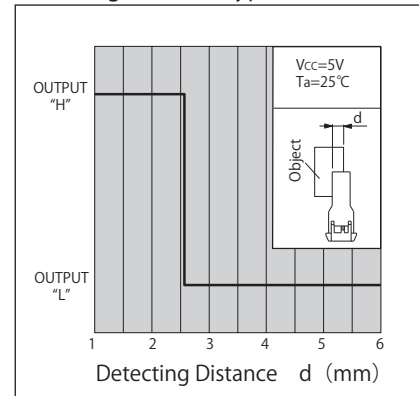
検出位置特性1 (代表例) KI5770 Detecting Distance (typ.)
