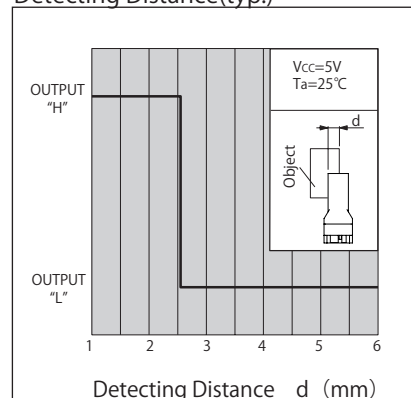
検出位置特性1 (代表例) KI3110 Detecting Distance (typ.)
