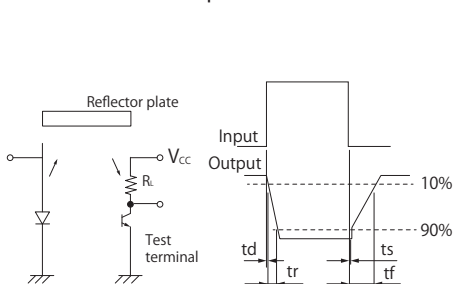
応答時間測定回路 Test Circuit for Response Time
