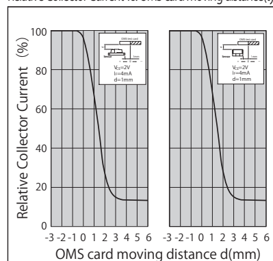
検出位置特性 X,Y (代表例) Relative Collector Current vs. OMS card moving distance (typ.)
