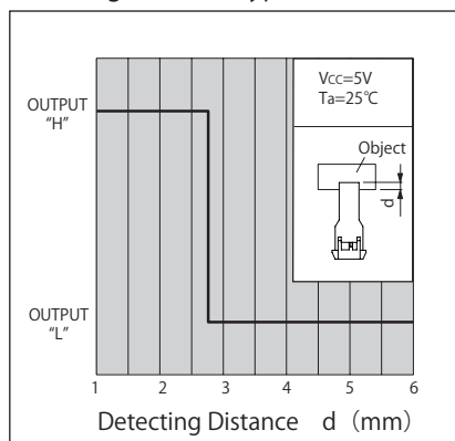
検出位置特性2 (代表例) KI5770 Detecting Distance (typ.)
