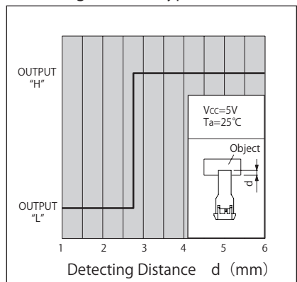
検出位置特性2 (代表例) KI5771 Detecting Distance (typ.)
