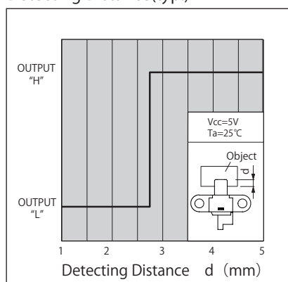
検出位置特性2 (代表例) KI5231 Detecting Distance (typ.)
