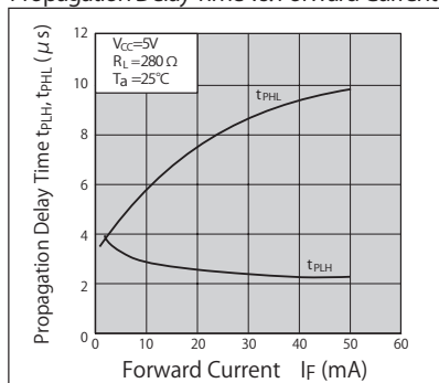
伝搬遅延時間—順電流特性 Propagation Delay Time vs. Forward Current
