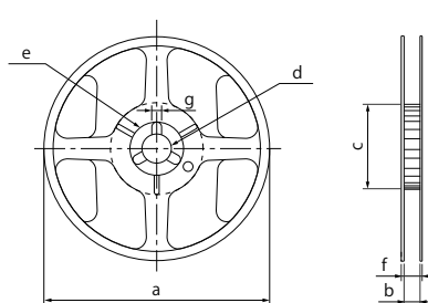
寸法表／Dimensions List
