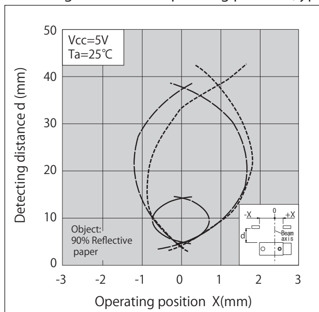
検出距離－動作位置特性2 (代表例) Detecting distance vs. Operating position (typ.)
