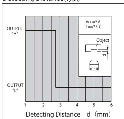
検出位置特性2 (代表例) KI3110 Detecting Distance (typ.)
